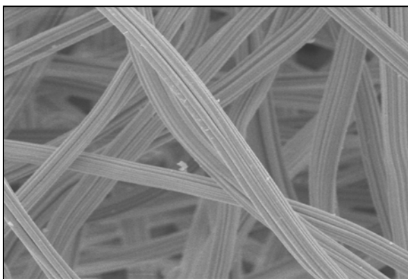
Hafnia Felt, Type HfF-50, originally at 1,000X
