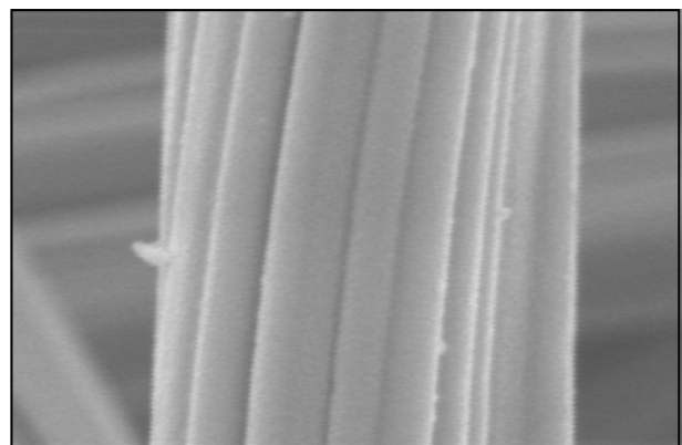
Hafnia Felt, Type HfF-50, originally at 10,000X
